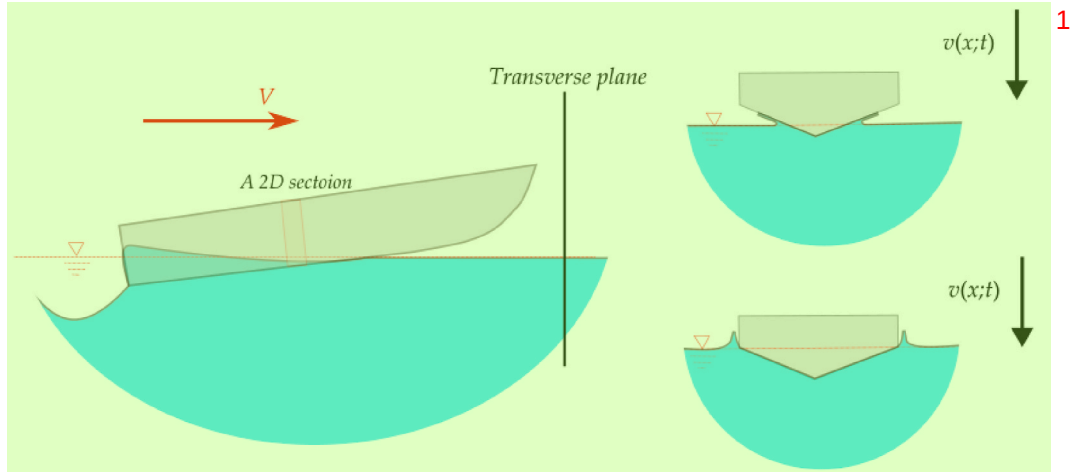
Fig. 12. A general overview of 2D + t theory. Two different stages of the water entry process, before and after chine wetting, are shown on the right side.
