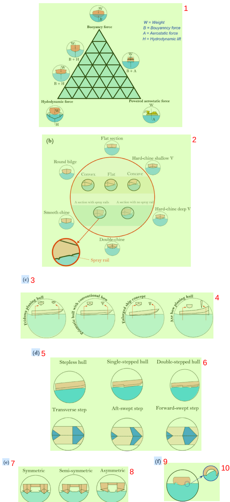
Fig. 2. (a) sustention triangle, (b) common sections of a mono-hull, (c) types of the bow section of a planing hull, (d) stepped hulls, (e) symmetric, semi-symmetric and asymmetric catamarans, and (f) planing trimaran.
