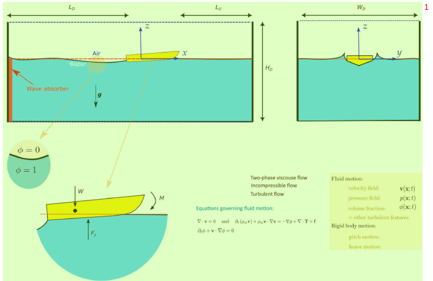
Fig. 14. General overview of a 3D CFD tank used for solving the fluid motion around a planing hull advancing in calm water condition. L_U and L_D are respectively upstream and downstream lengths and W_D is the width of domain. The air-water interface is captured via a VoF (two-phase) model.
