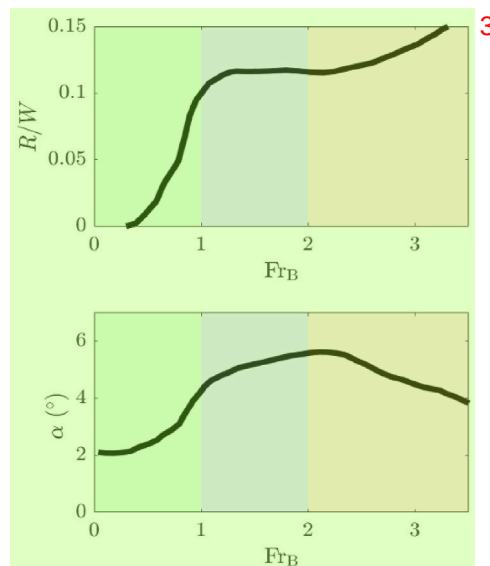
Fig. A1. An example of resistance versus beam Froude Number and trim angle versus Froude Number curves. Data is extracted from Fridsma (1969).
