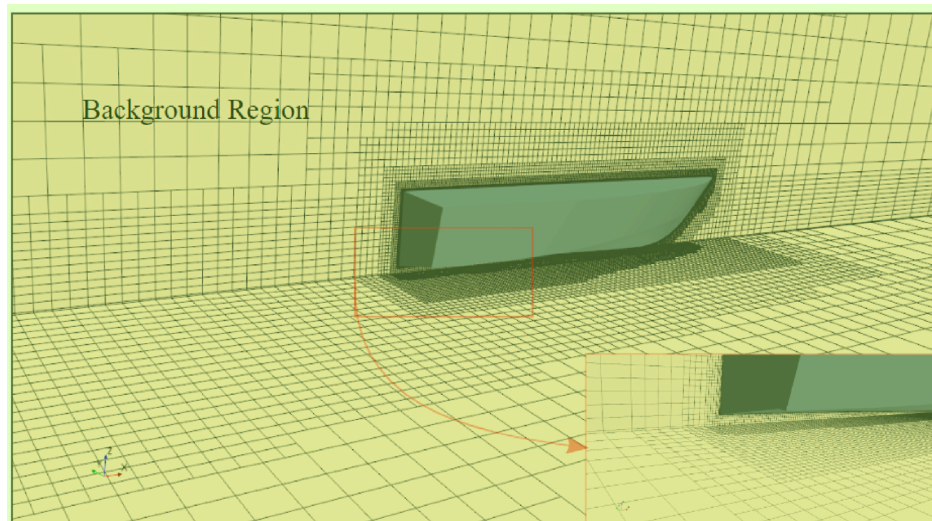
Fig. 15. An example of CFD mesh around a planing hull free in heave and pitch directions, Hosseini et al. (2021).
