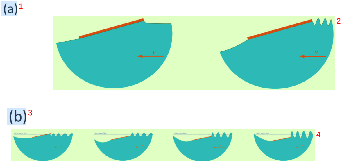
Fig. 7. Demonstration of Tuck model (Tuck, 1982b) - (a) surface tension may lead to the generation of waves in front of the planing plate; (b) the decrease of immersion depth in way of the leading edge of the planing plate may decrease the generated waves.
