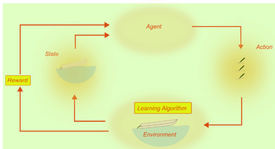
Fig. 23. The general framework of RL for control of a planing boat. Here a trim tab is supposed to be the control device and state represents the boat motions and positions.
