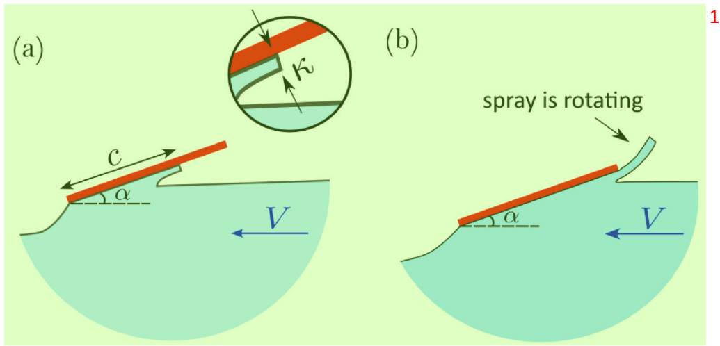
Fig. 6. A planing plate exposed to steady flow. In (a) the jet flow is formed but is not rotating. In (b) spray is rotating, while it is thicker than the spray formed in (a).
