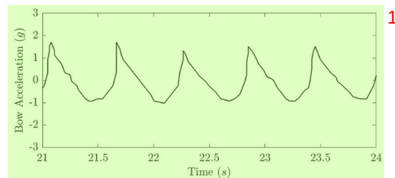
Fig. A2. An example of time history of vertical acceleration at bow of a planing hull. Data is extracted from Garne (2005). . 2
