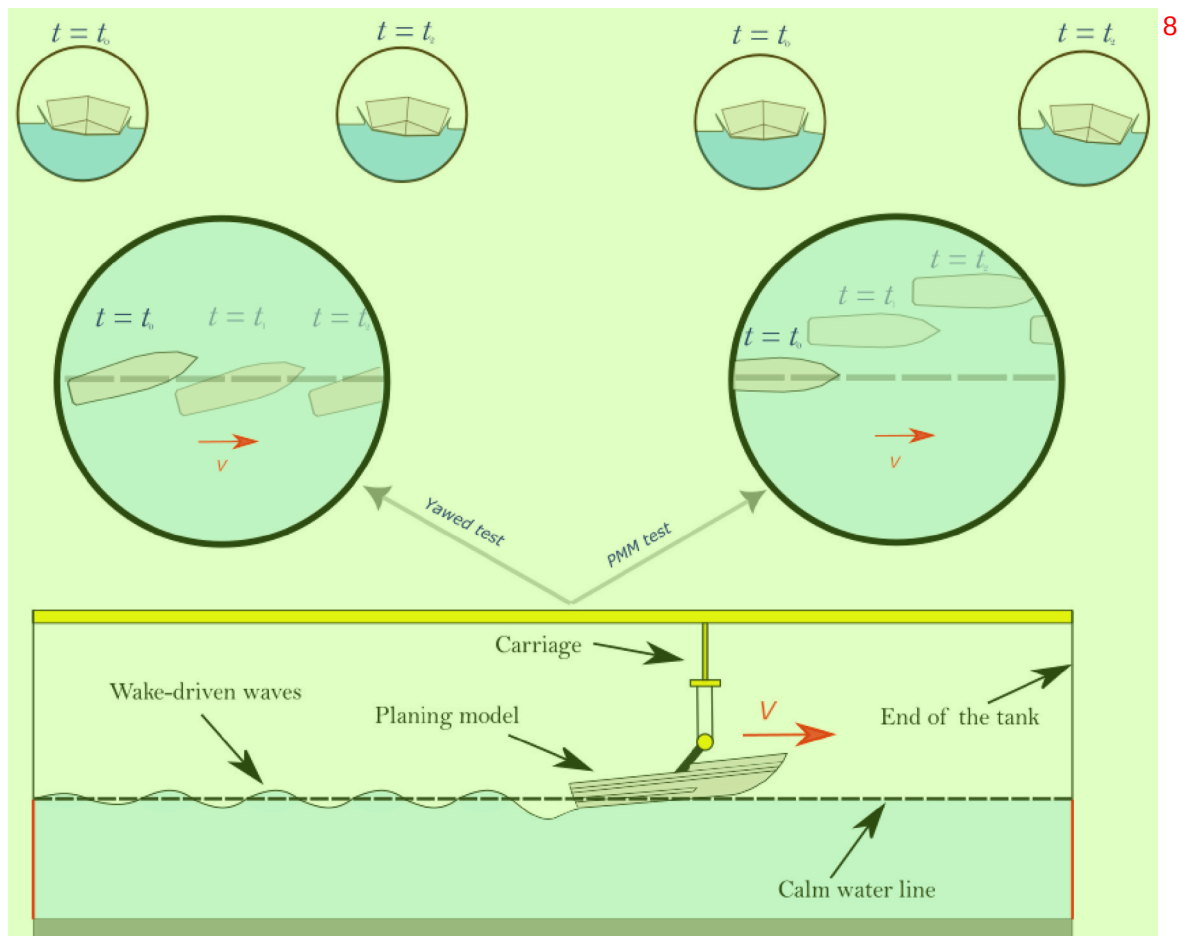
Fig. 5. General schematics of yawed and PMM tests in tanks. 9
