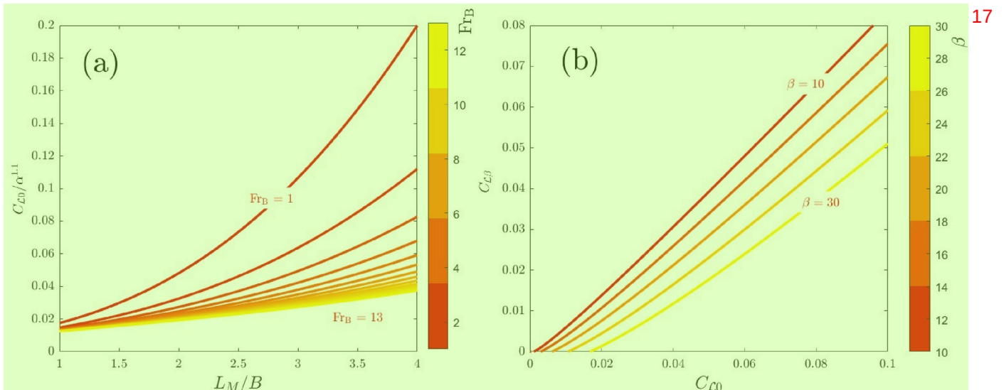
Fig. 9. Lift force variation according to Savitsky (1964).
